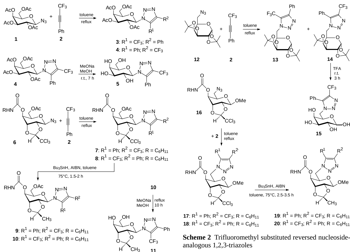
Scheme 1 Trifluoromethyl substituted nucleoside-analogous 1,2,3-triazoles
