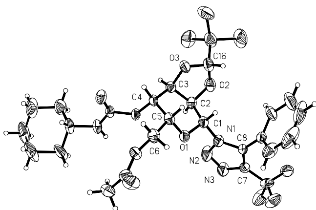
Fig. 2 X-ray structure of 1-[6- O -acetyl-4- O -cyclohexylcarbamoyl-2,3- O -(2,2,2-trichloroethylidene)- \beta -D-gulopyranosyl]-4-trifluoromethyl-5-phenyl-1,2,3-triazole ( 7 ); 30% probability of the terminal ellipsoids.
